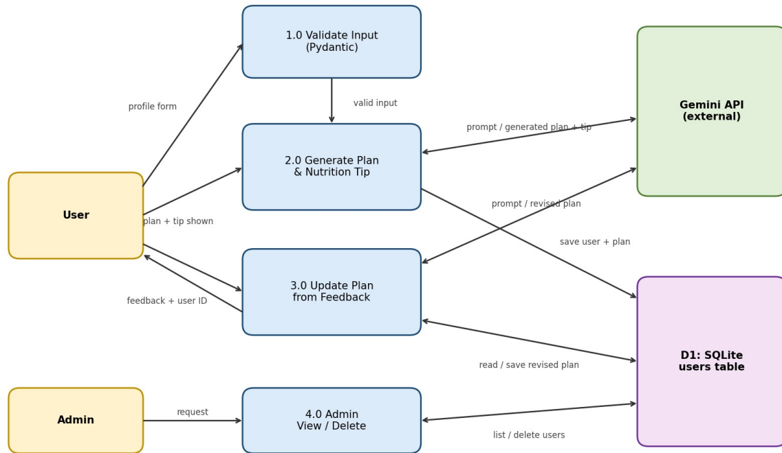
FitBuddy – Data Flow Diagram (Level 1)
